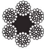
6 x 36 WARRINGTON SEALE WITH FIBER CORE
