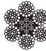
6 x 36 WARRINGTON SEALE WITH IWRC
