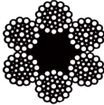
6 x 36 WARRINGTON SEALE WITH FIBER CORE
