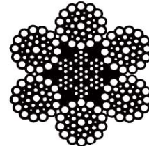
6 x 36 WARRINGTON SEALE WITH IWRC
