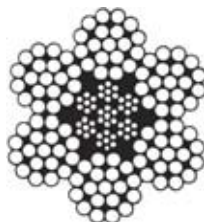
6 x 19 (1 + 6 + 12) WITH IWRC
