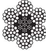
6 x 25 FILLER WIRE WITH IWRC
