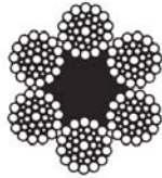
6 x 36 WARRINGTON SEALE WITH FIBER CORE
