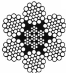
6 X 31 WARRINGTON SEALE WITH IWRC
