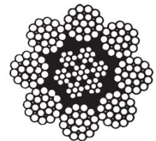
8 x 25 SPIN RESISTANT WITH IWRC
